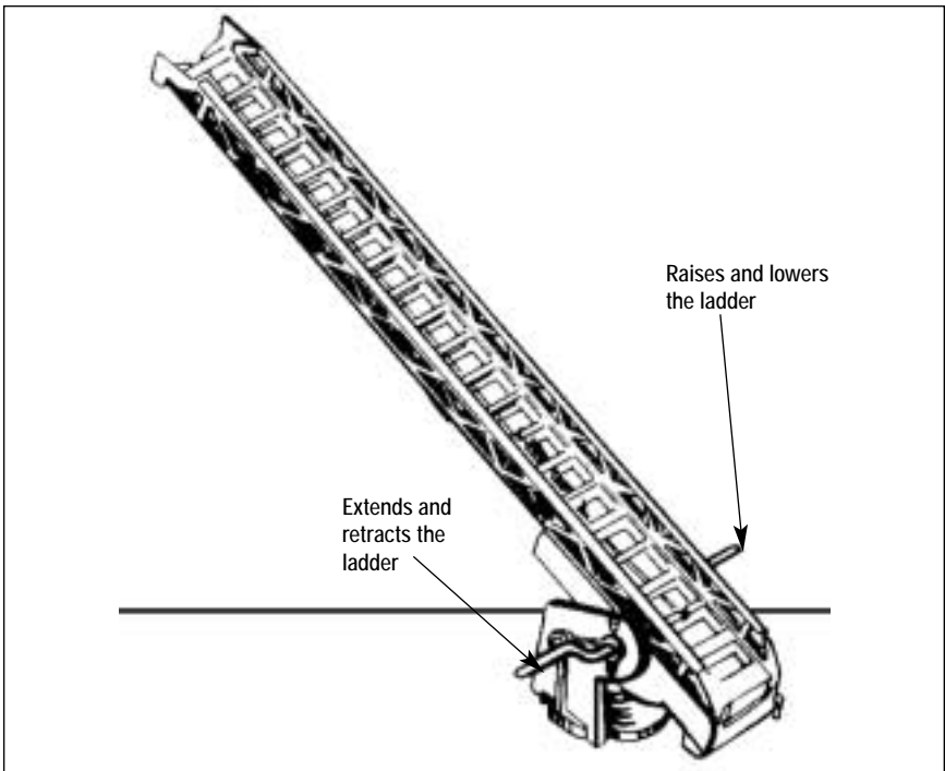
Figure 1. Ladder operation
