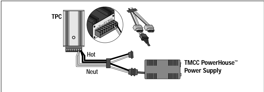
Figure 1. Powering the TPC with one PowerHouse™ Power Supply
