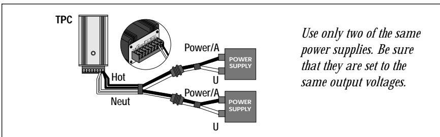
Figure 3. Powering the TPC with two transformers
