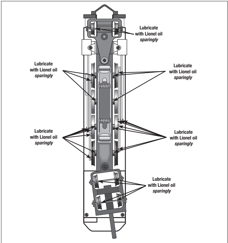
Figure 15. Locomotive lubrication points
