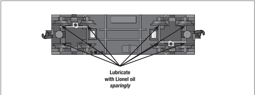
Figure 16. Tender lubrication points
