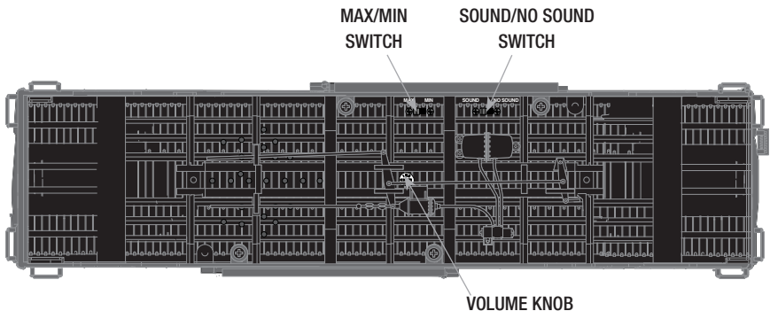
Figure 1. Switch locations
