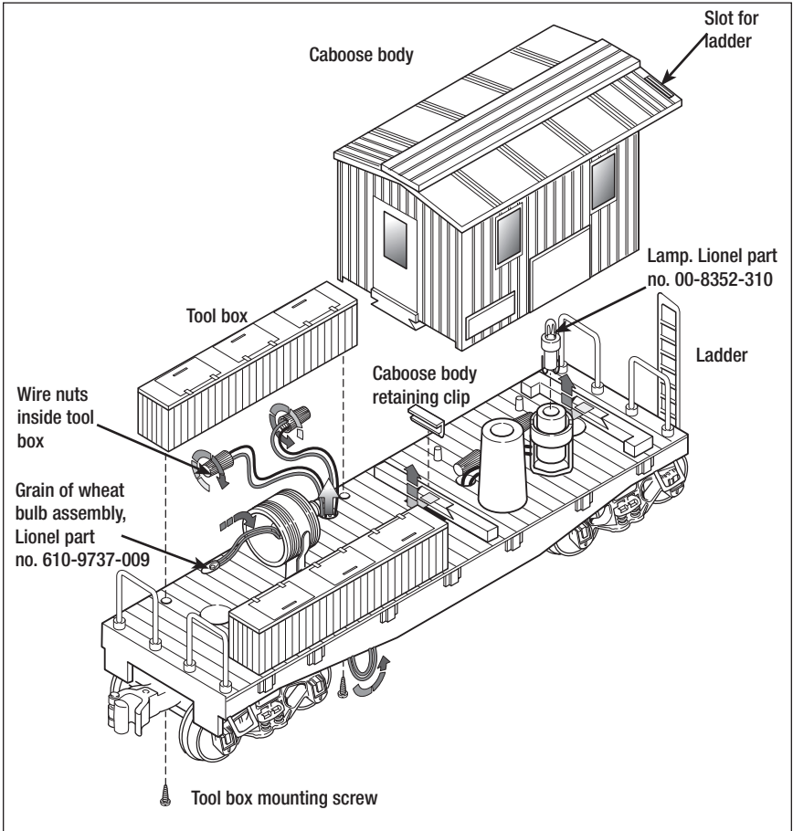
Figure 1. Assembly
