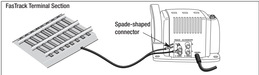
Figure 3. Thumbscrew connections
