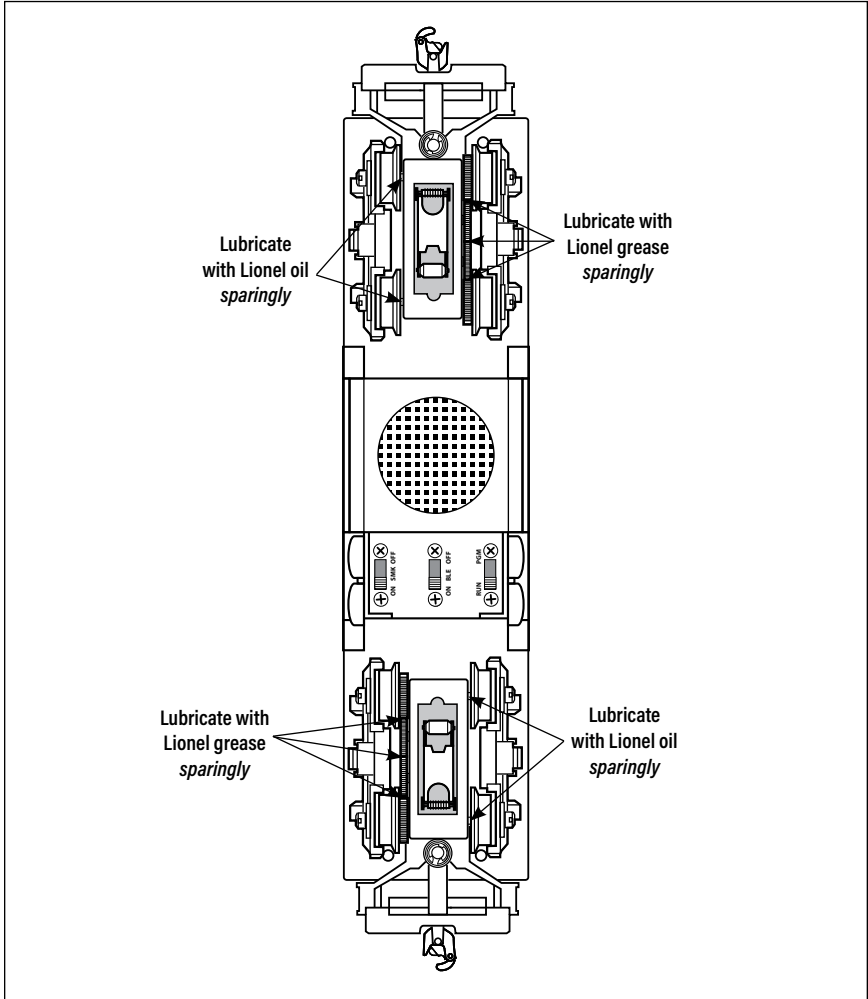
Figure 9. Locomotive lubrication points
