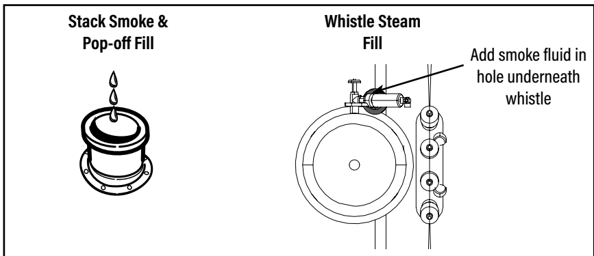
Figure 6. Smoke fluid fill locations
