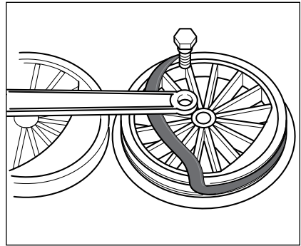
Figure 19. Replacing traction tires
