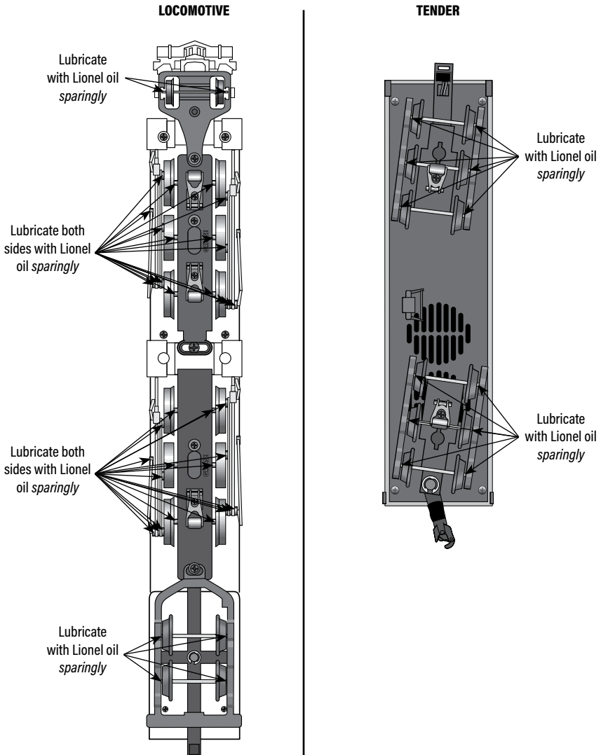
Figure 18. Locomotive and tender underside details and lubrication points
