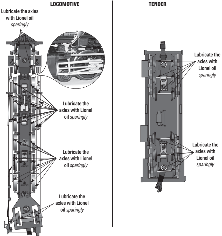
Figure 17. Locomotive and tender underside details and lubrication points
